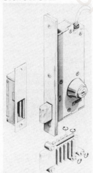
Motorslot.
